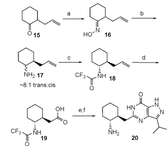
Scheme 2. Reagents and conditions: (a) \text{NH}_2\text{OH} \cdot \text{HCl} , pyridine, EtOH, rt; (b) Li, \text{NH}_3 , THF, tBuOH, -78^\circ\text{C} ; (c) \text{CF}_3\text{CO}_2\text{Me} , \text{CH}_2\text{Cl}_2 ; (d) \text{KMnO}_4 , \text{NaIO}_4 , acetone, water; (e) 2 , T3P, \text{Et}_3\text{N} , EtOAc, rt; (f) \text{KOrBu} , 1-propanol, 80^\circ\text{C} .
