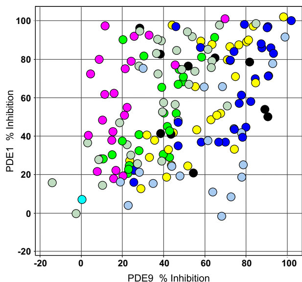
Figure 2. Profile of directed 2nd array in PDE 1 and 9 assays (1 \mu M concentration). Colored by R^1, R^3 : ● H, cPent; ● H, iBu; ● H, iPr; ● H, nBu; ● H, tBu; ● H, pyridin-2-yl; ● H, pyridin-3-yl; ● Me, nPr.
