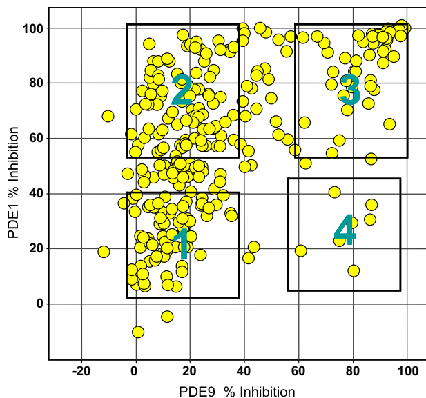
Figure 1. Profile of diverse 1st array in PDE 1 and 9 assays (1 \mu M concentration).
