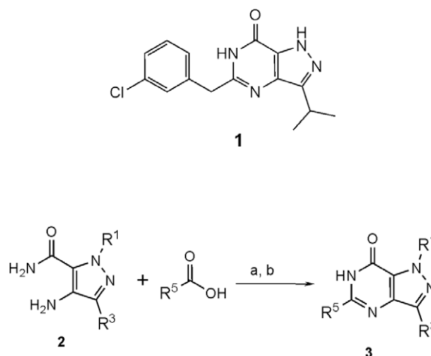
Scheme 1. Reagents and condition: (a) CDI, pyridine, DMA; (b) KOtBu, IPA, 80 °C.
